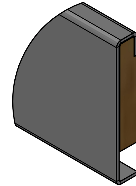
DETAIL B NO END CAP SCALE 12" = 1'-0"
